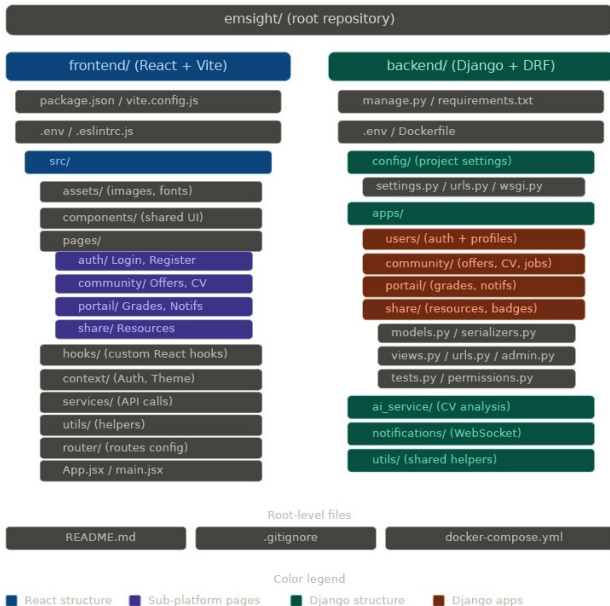
FIGURE 1 – Architecture Générale et Technique
