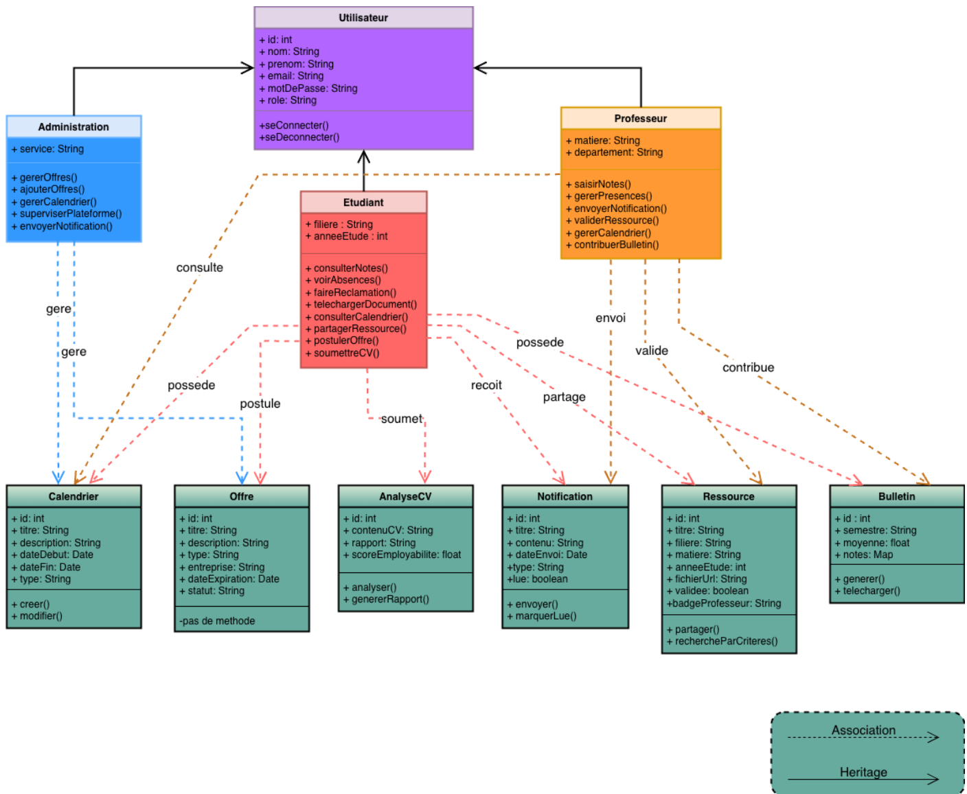
FIGURE 4 – Diagramme de classes
